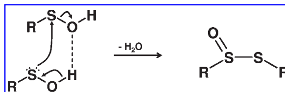
FIG. 1. Self-condensation of two sulfenic acid molecules forming a thiol-sulfinate.
